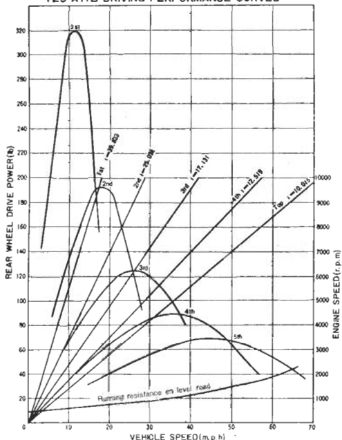
125 AT1B DRIVING PERFORMANCE CURVES
