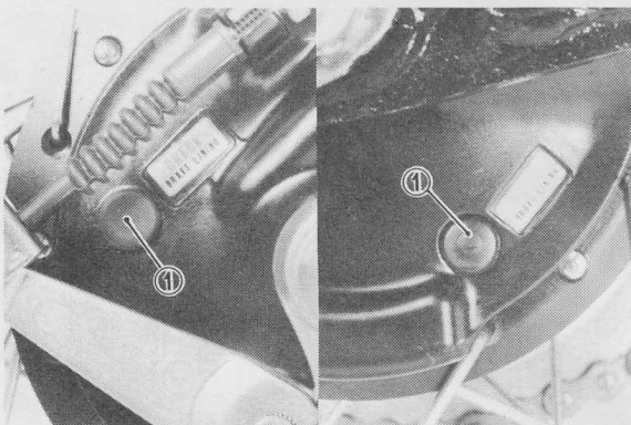
1. Inspection hole
