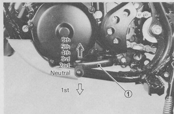
1. Change pedal
