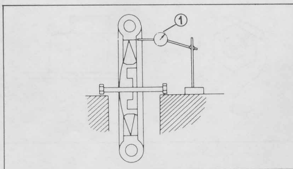
1. Dial gauge
