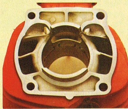
New 1979 cylinder porting.
