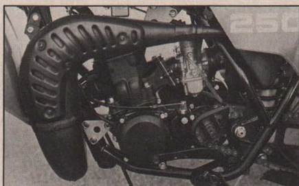
The KXT is the first production water-cooled three-wheeler, and the experiment seems to have paid off. L/C cylinder delivers more horsepower than ATC250.
