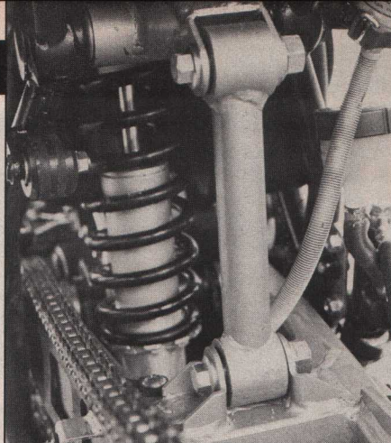
Single-strut Uni-Trak is a dead ringer for the motorcycle version. Rebound damping is adjustable.
