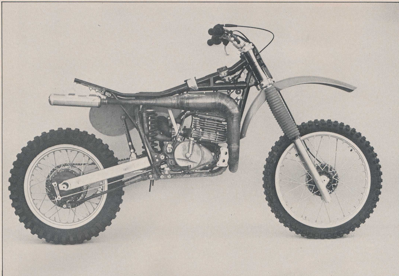
Frame has heavy-duty backbone. Pipe is handmade.
