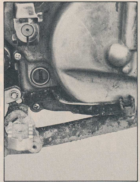
Footpegs are machined from billet aluminum. Brake pedal has folding tip. Transmission oil can be checked by looking through the sight gauge.
