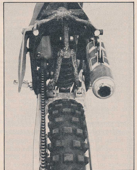
Whole unit sets to right of chassis, making room for chain and air cleaner.
