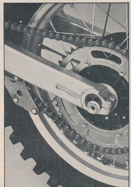
Aluminum swing arm is 23 in. long and features eccentric axle adjusters.
